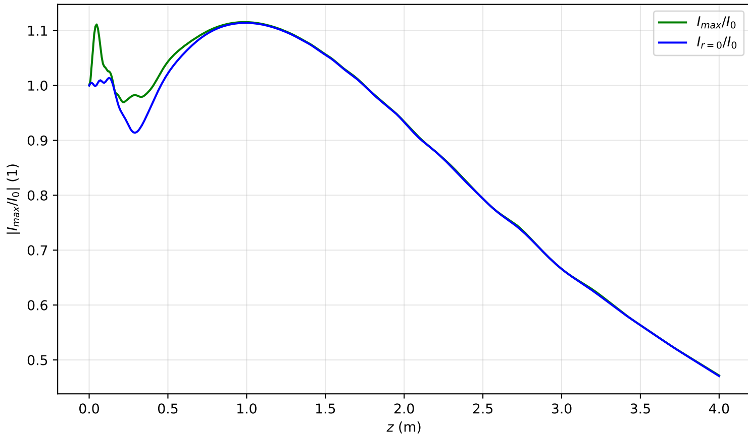
I_{max}(x = 0, y = 0, z)/I_0 , P_{in}=0.6P_{cr} , noisy input, artificial time
